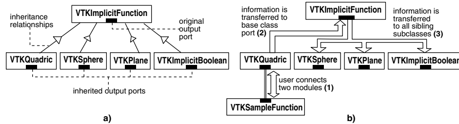
Fig. 7. Effect of object-orientation on SMARTLINK
