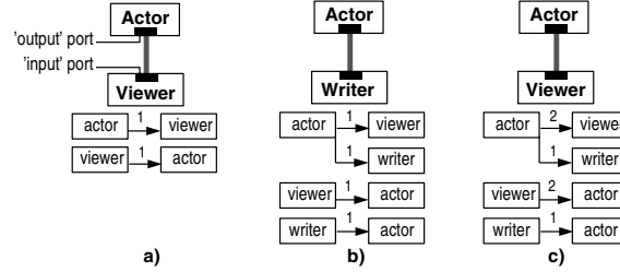
Fig. 2. SMARTLINK database for three network construction stages
