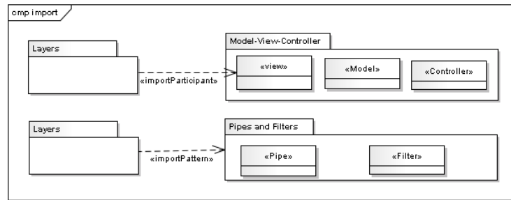
Figure 5. importPattern and importParticipant relationships among pattern participants
