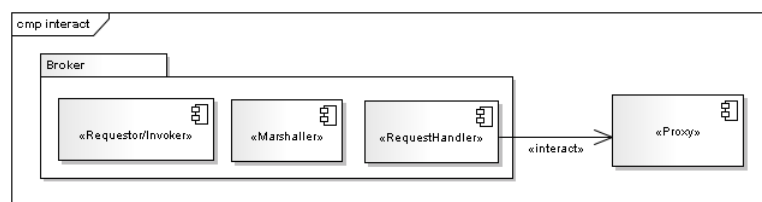
Figure 6. The interact relationship
