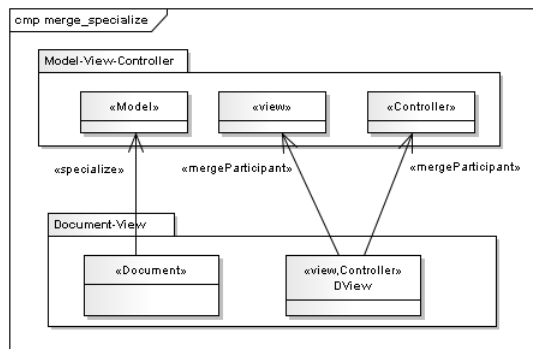
Figure 2. The mergeParticipant relationship
