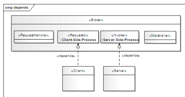
Figure 4. The depends relationship among pattern participants
