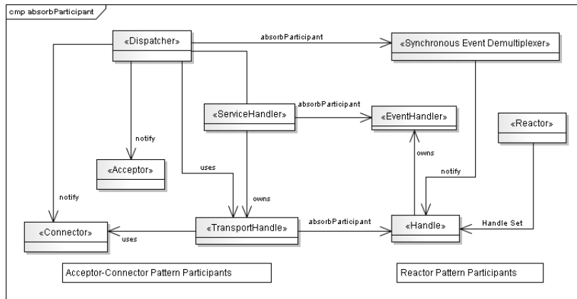
Figure 1. The absorbParticipant relationship between Reactor and Acceptor-Connector
