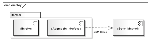
Figure 3. Employ relationship between the Iterator and Batch Method Patterns
