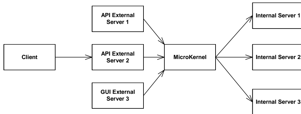
Figure 9: Microkernel example
