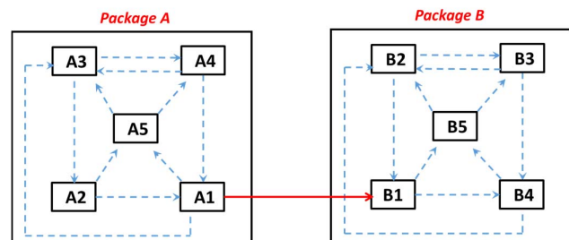
Fig. 1. Aggregation of metrics to the architecture level
