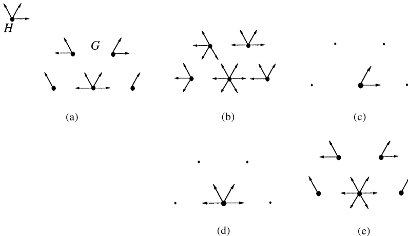
Fig. 2. Morphological operations on the motion group \mathbf{M} : (a) set G , structuring element H ; (b) dilation of G by H ; (c) erosion of G by H ; (d) opening of G by H ; (e) closing of G by H .
