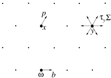
Fig. 1. Representation of elements of the Euclidean motion group on the hexagonal grid. b : base-pointer. p : pointer with base-point x . \tau_y \Sigma : the collection of group elements which map the origin \omega to y . Each pointer represents a unique group element.
