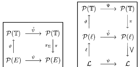
Fig. 6. Left: relations between mappings on \mathcal{P}(E) and \mathcal{P}(\mathbb{T}) . Right: relations between mappings on \mathcal{L}, \mathcal{P}(\ell) and \mathcal{P}(\mathbb{T}) .
