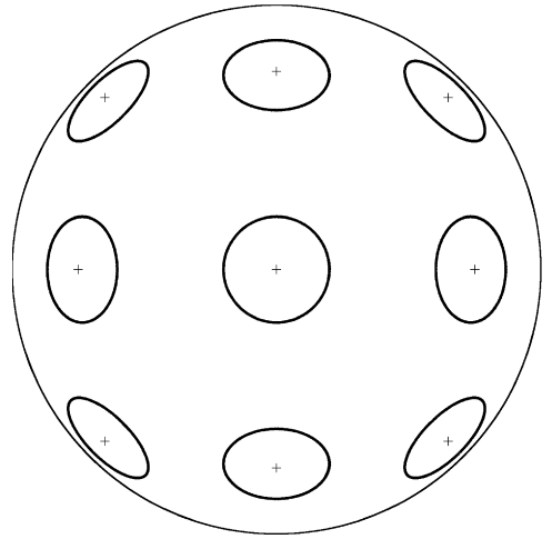
Fig. 13. Disc C centered at the origin of D , and its ‘translates’ C_{x,y} corresponding to rotated discs on the sphere under orthographic projection. A ‘+’ sign indicates the projection of the center of a rotated disc.
