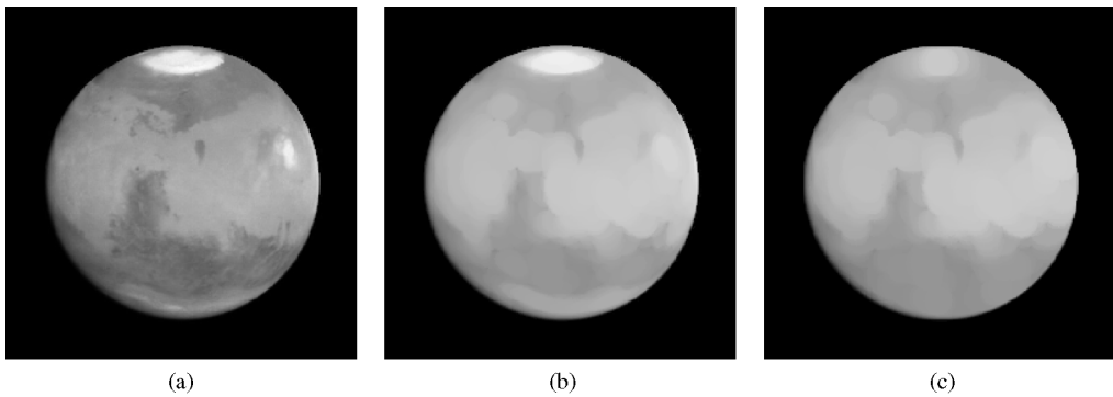
Fig. 14. (a) Picture of the planet Mars (for details, see text), (b): spherical grey-scale opening, (c) Euclidean grey-scale opening.
