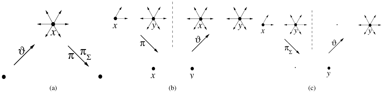
Fig. 5. Illustration of properties of \pi, g, \pi_\Sigma : (a) \pi g = \pi_\Sigma g = \text{id}_{\mathcal{P}(E)} . (b) g \pi = \delta_\Sigma^zeta . (c) g \pi_\Sigma = \tilde{zeta}_\Sigma^zeta .
