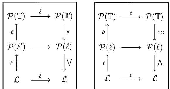
Fig. 12. Construction of a \mathbb{T} -dilation \delta (left), and a \mathbb{T} -erosion \varepsilon (right), on a lattice \mathcal{L} with sup-generating family \ell and inf-generating family \ell' .
