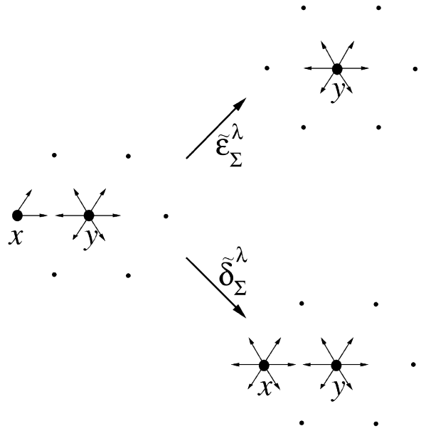
Fig. 3. Action of the erosion and dilation by \Sigma on a subset of \mathbb{M} .
